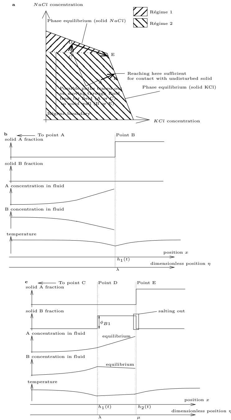
Figure 10. a : Schematic of path in (salt A concentration, salt B concentration) space traced out, on moving from far-field fluid (point A) to single front (point B) or from far-field fluid (point C) past trailing front (point D) to leading front (point E), for pure KCl solid, with effect of temperature on phase-equilibrium concentration neglected. b : Schematic illustration of solid fractions, concentrations, and temperature, as functions of position, without salting out. c : Schematic illustration of solid fractions, concentrations, and temperature, as functions of position, with salting out.
