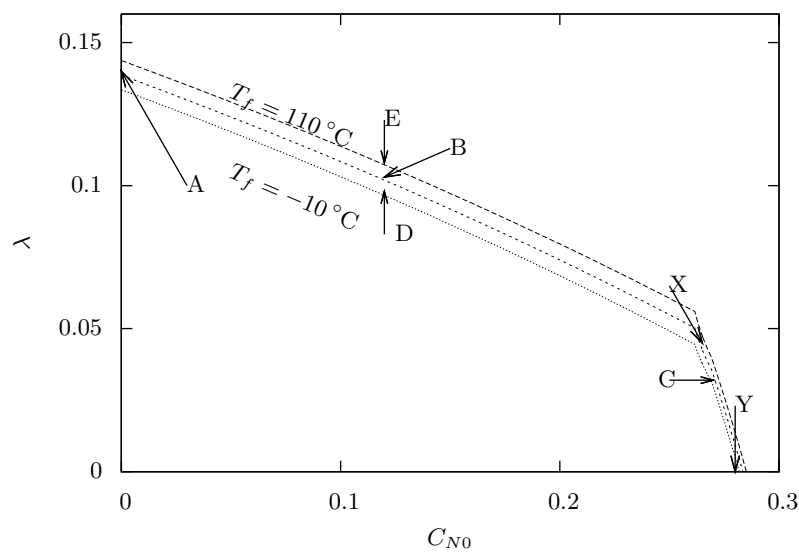
Figure 4. This graph shows predictions for the dissolution rate of solid KCl ( k = K ,) as a function of NaCl concentration in the far-field brine; C_{N0} represents the externally-imposed concentration of the far-field brine, not the local concentrations influenced by the dissolving solid. Three curves are plotted, corresponding to far-field brines at T_f = -10^\circ C , T_f = 50^\circ C , and T_f = 110^\circ C . Throughout, the KCl concentration of the far-field brine is C_{K0} = 0 , and the far-field solid temperature is T_s = 50^\circ C .
