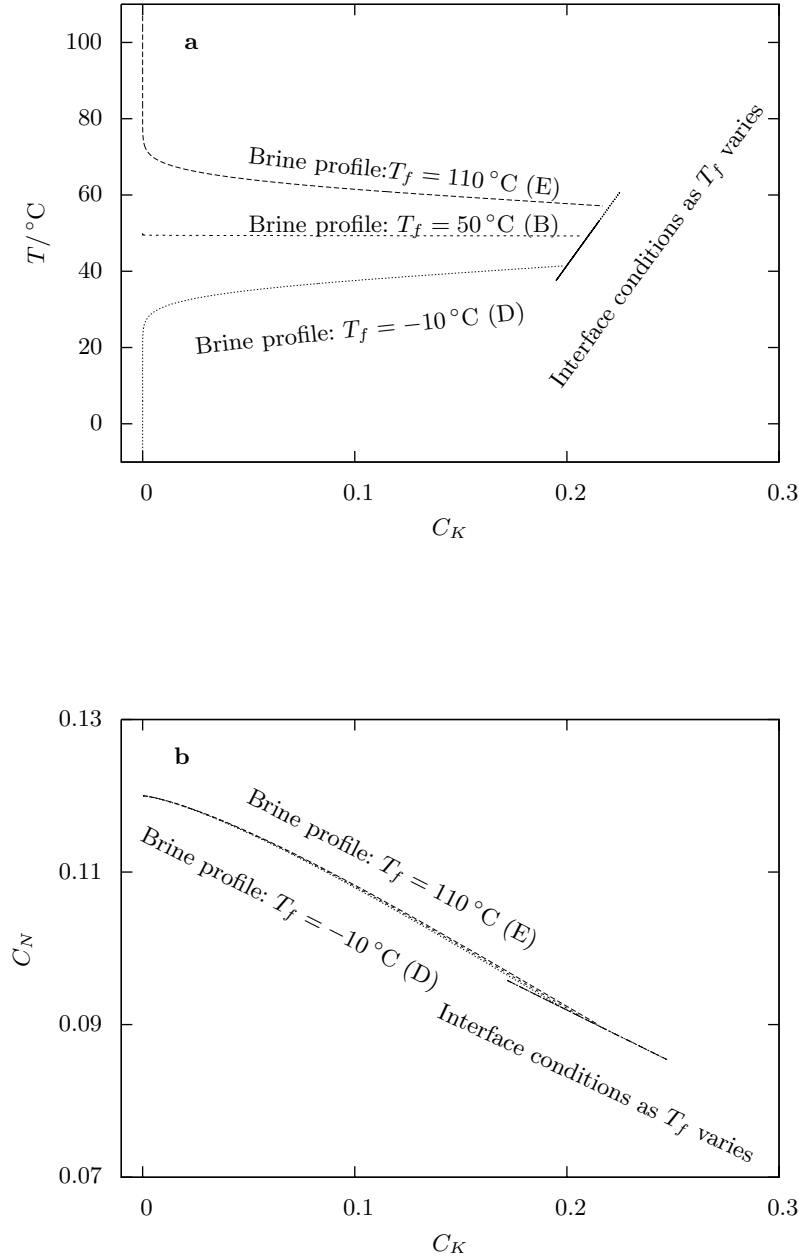
Figure 6. a: this graph shows predicted KCl concentration-temperature profiles of the brine, for three far-field brine temperatures (points D, B, and E in figure 4,) along with the predicted locus, in KCl concentration-temperature space, of interface brine conditions, as T_f varies. b: this graph shows predicted KCl concentration- NaCl concentration profiles of the brine, for three far-field brine temperatures (points D, B, and E in figure 4,) along with the predicted locus, in KCl concentration- NaCl concentration space, of interface brine conditions, as T_f varies. Both panels: the only solute in the far-field brine is NaCl ( C_{K0} = 0 .) The solid is KCl ( k = K .) The far-field brine NaCl concentration C_{N0} = 0.12 and the far-field solid temperature T_s = 50^\circ\text{C} .
